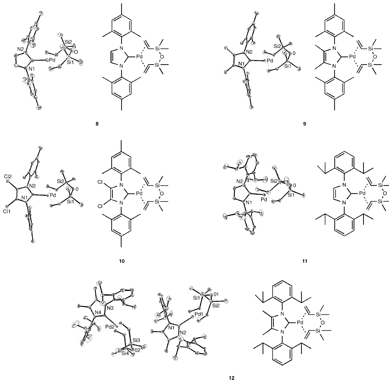
Figure 1. Monocarbene-palladium(0)-dvds complexes 8–12 . Hydrogen atoms are omitted for clarity; the thermal ellipsoids correspond to 30% probability.
